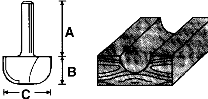
Cove Box Bits
