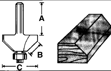
45° Chamfer Bits with Bearings (Can 45° bevel boards from 6mm thick (RBA138) to 18mm thick (RBA340))
