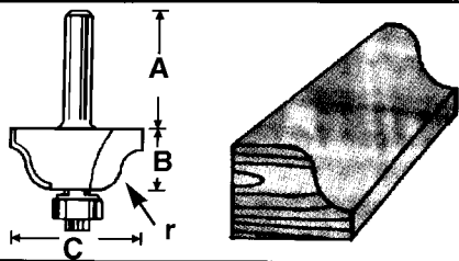
Roman Ogee Bits with Bearings
