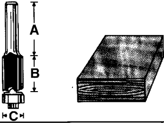
Two Flute Flush Trim Bits with Bearings (For flush trimming laminates)
