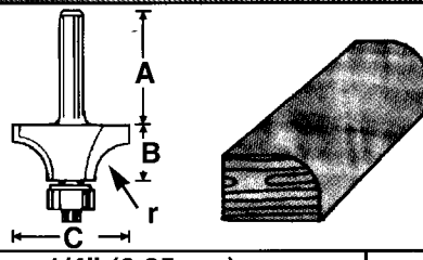
Corner Rounding Bits with Bearings (can also create a stepped radius by adjusting cutter height)
