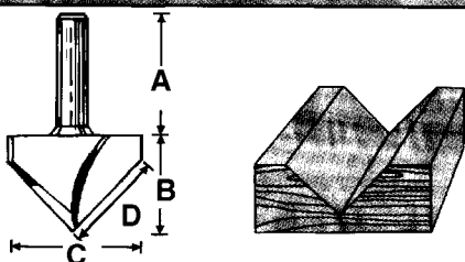
V-Groove Bits (Can 45° bevel boards from 8mm thick (RBA154) to 12mm thick (RBA354))
