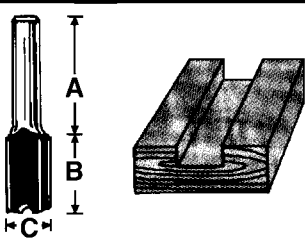
Two Flute Straight Bits (For grooving, edge planing, rebating & morticing)
