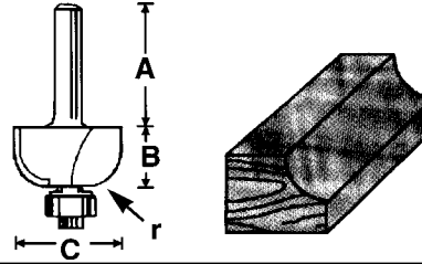
Cove Bits with Bearings Radius (r) - 9.5mm
